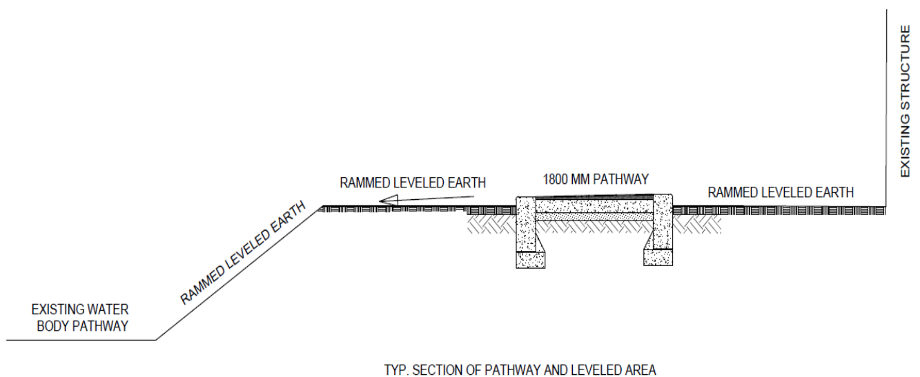
Typ, section of pathway and leveled area
