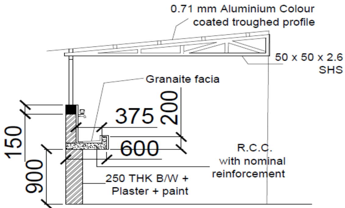
Section and Elevation
