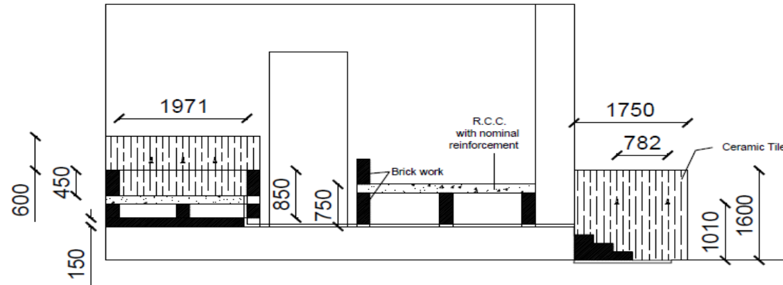
Section and Elevation
