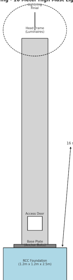
GA Drawing - 16 Meter High Mast Light Pole
