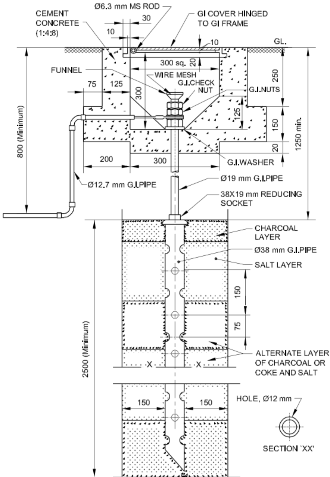
PIPE EARTHING
